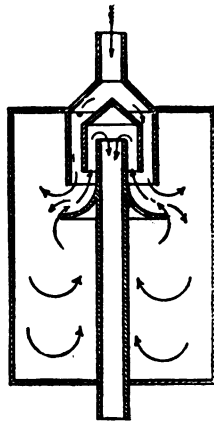
FIG. 16.—Thompson Muffler.
